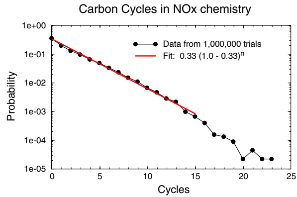
Fig. 13. Distribution of carbon cycles in NO x chemistry.
