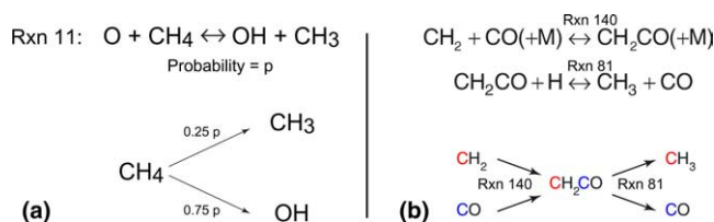
Fig. 17. Examples of reactions involving molecules with several of the atoms being tracked. Example (a) shows a symmetric case involving H atoms in CH_4 . Example (b) show an unsymmetrical case involving carbon.
