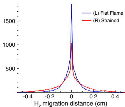
Fig. 9. Symmetrized distributions of horizontal \text{H}_2 migration show how the flowfield strain disrupts local hydrogen chemistry in the rich flame.
