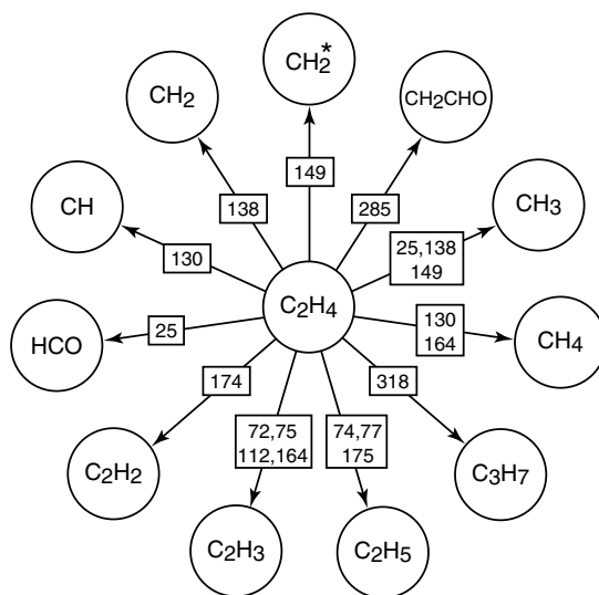
Fig. 1. State-transition diagram for ethylene, including numbered reactions from the GRI-Mech 3.0 kinetics mechanism [11], illustrating the chemical reactions that shift carbon atoms to other molecules.
