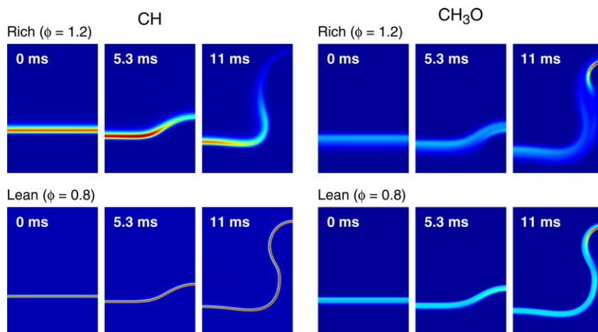
Fig. 5. Behavior of CH and \text{CH}_3\text{O} during vortex–flame interaction for \phi = 0.8 and 1.2.
