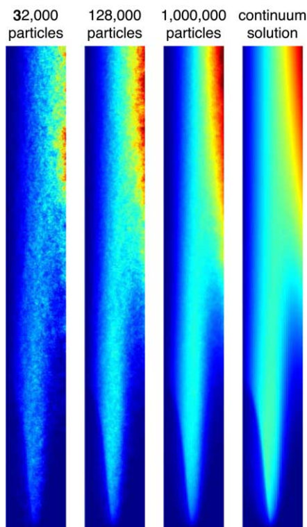
Fig. 12. NO concentration in moles/area comparing 32,000, 128,000 and 1,000,000 particles with the continuum solution.
