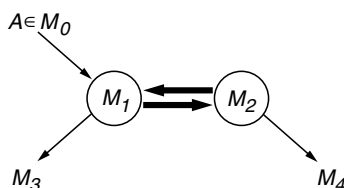
Fig. 15. Two species ( M_1 and M_2 ) with rapid forward and backward reactions near equilibrium. If tracked particle A \in M_0 enters the M_1 species group, the probability that A will emerge later in the M_4 group depends on whether the production rates between M_1 and M_2 are coalesced.
