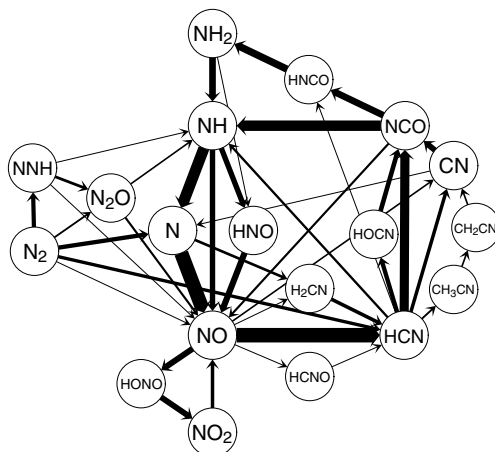
Fig. 11. Reaction path diagram for nitrogen chemistry. Only edges at least 3% of the strongest are shown.
