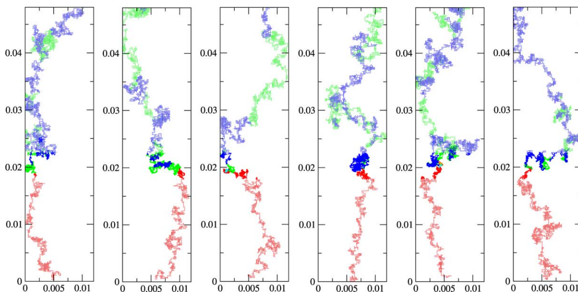
Fig. 2. Carbon trajectories for flat laminar premixed flame, \phi = 1.2 .
