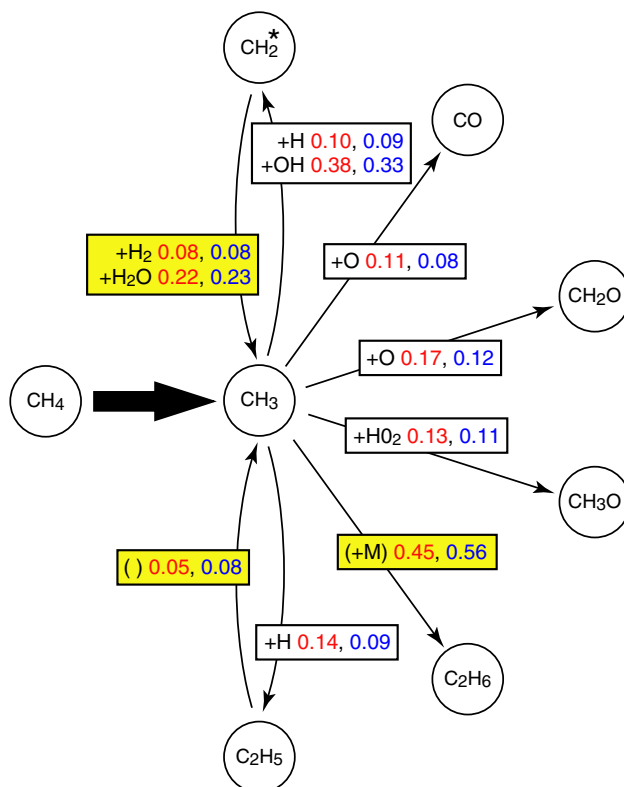
Fig. 8. Dominant chemistry of \text{CH}_3 in the \phi = 1.2 case, determined from stochastic particle analysis. Each pathway is annotated with the associated reaction partner(s) and strength, normalized to the net number of \text{CH}_4 \rightarrow \text{CH}_3 events. The red values represent statistics of particles released on the left, the blue values from particles release on the right. Only paths of strength >5\% are shown. Pathways not involving radical partners are highlighted yellow, and are increased in the side interacting with the vortex over those in the unperturbed side. All \text{CH}_3 destruction reactions involving radicals are weaker in the strained flame region, and in particular paths leading to \text{CH} through the \text{CH}_2(\text{s}) molecule are reduced while those leading to the \text{C}_2 branch through \text{C}_2\text{H}_5 and \text{C}_2\text{H}_6 are enhanced. (For interpretation of the references to color in this figure legend, the reader is referred to the web version of this article.)
