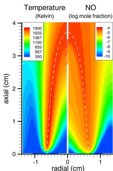
Fig. 10. Temperature and NO mole fraction for the laminar nonpremixed flame. The dotted white line is the stoichiometric boundary between the fuel and air.
