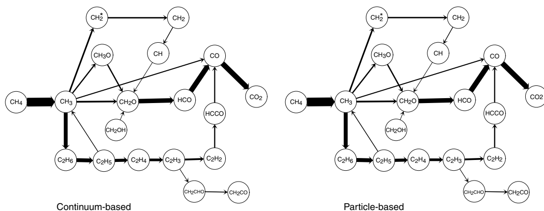
Fig. 3. Reaction path diagrams for rich ( \phi = 1.2 ) premixed methane flame computed using PREMIX with GRI-Mech 3.0: continuum-based CHEMKIN rate evaluation, and particle-based tabulation of 80,000 trajectories.
