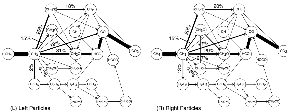
Fig. 6. Carbon reaction path diagrams for vortex–flame interaction, \phi = 0.8 . Here only paths of strength >1\% of the largest path, \text{CH}_4 \rightarrow \text{CH}_3 , are shown. For some paths of interest their weights are shown as a percent of the strongest.
