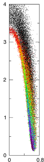
Fig. 14. Location of initial reaction for exiting NO x particles. Black points mark initial reaction locations for particles that do not participate in carbon recycling. The remaining points are color-coded to indicate the number of carbon cycles in the particle history using a rainbow palette ranging from red (=1) to violet ( \geq 12 ).
