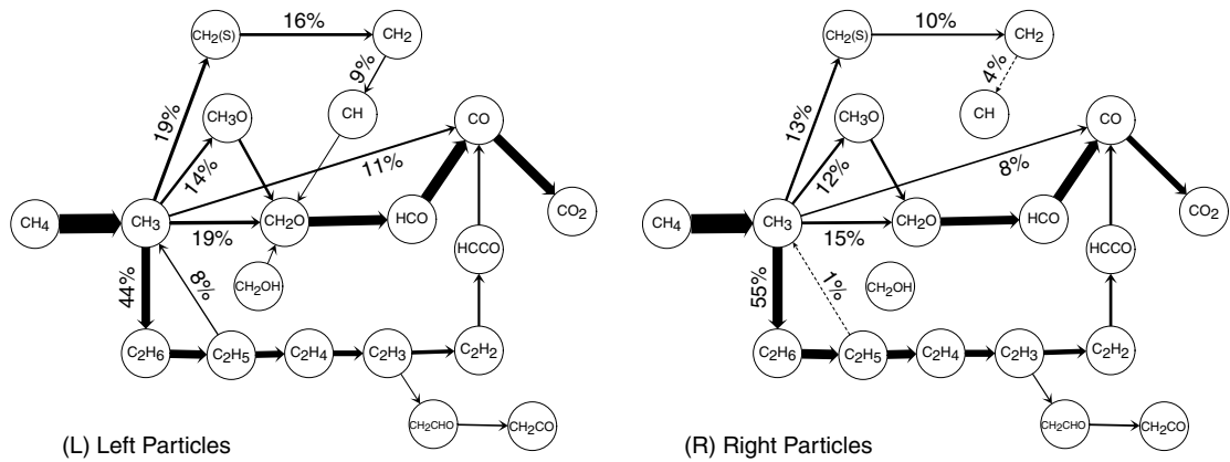
Fig. 7. Carbon reaction path diagrams for vortex–flame interaction, \phi = 1.2 . Here only paths of strength >5\% of the largest path, \text{CH}_4 \rightarrow \text{CH}_3 , are shown. For some paths of interest their weights are shown as a percent of the strongest.
