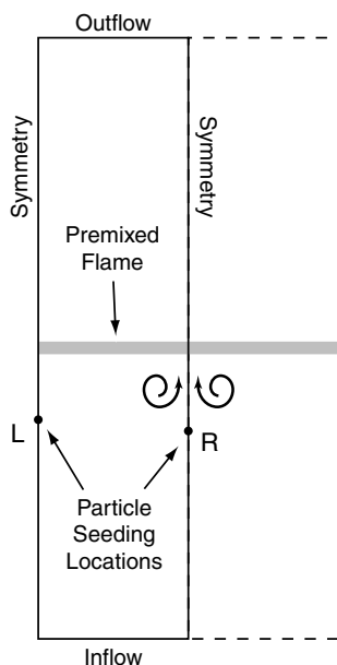
Fig. 4. Schematic of the premixed methane flame–vortex problem. The shaded line represents the position of the flame, and the swirl lines represent the initial vortex. We impose symmetry along the sides of the 1.2 \times 4.8 cm domain to avoid modeling the dotted region.
